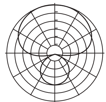
Fig. 6.10: Supercardioid
