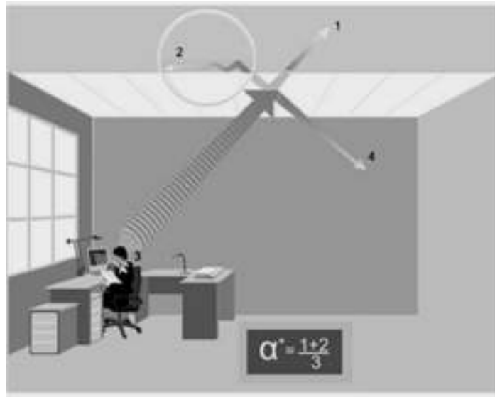
Fig. 1.4: Absorption coefficient
