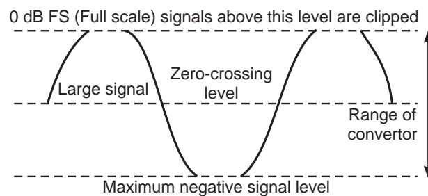
Fig. 3.7: Clipping of signal
