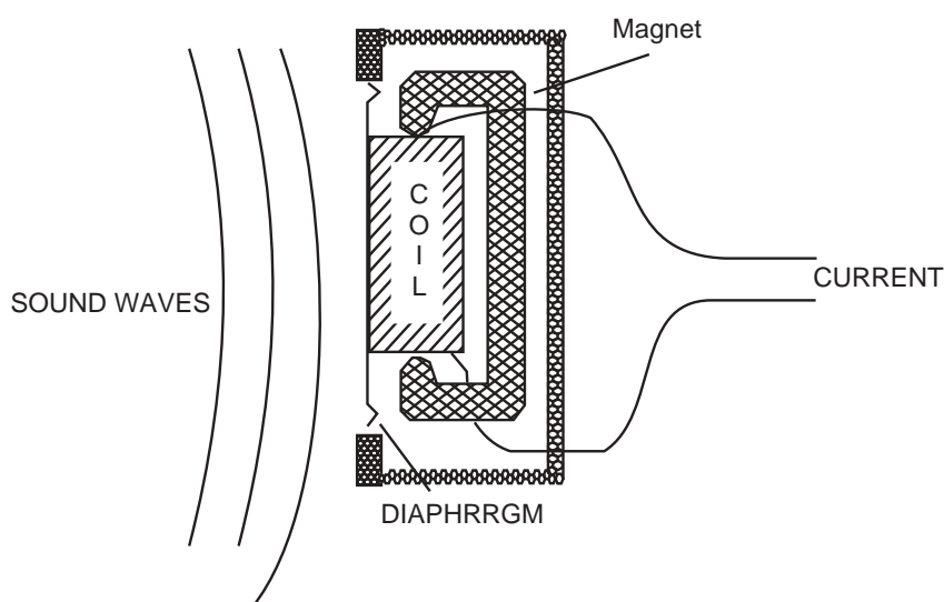
Fig. 6.2: Dynamic microphone
