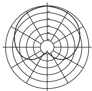
Fig. 6.8: Cardioid
