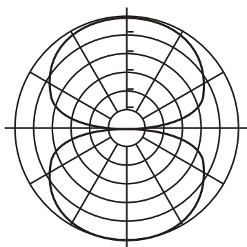
Fig. 6.6: Bi-directional
