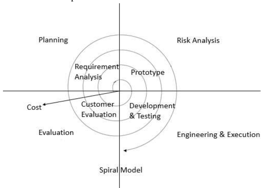
Figure 8: Spiral Model
