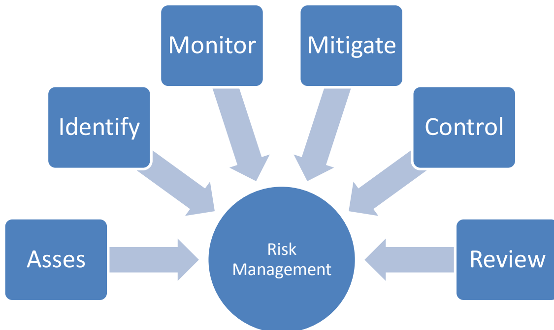
Figure 2: Risk management
